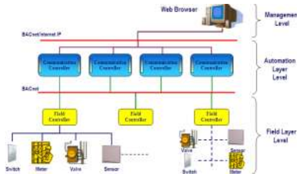
Fig.1. the fundamental structure of building management system
