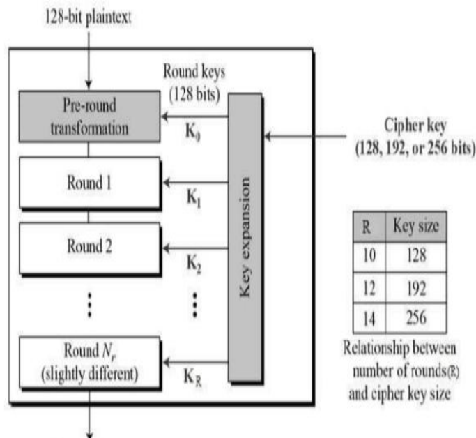
Fig 1: AES Algorithm
